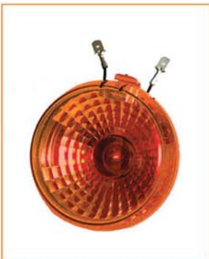
N520 Hella circular amber indicator lamp 90mm 1 x 12v 21w Single Contact (D481)
